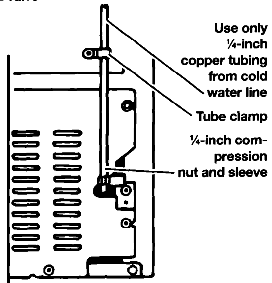
Style #2 valve
