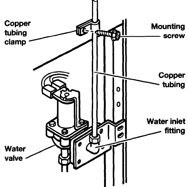
Style #1 valve
